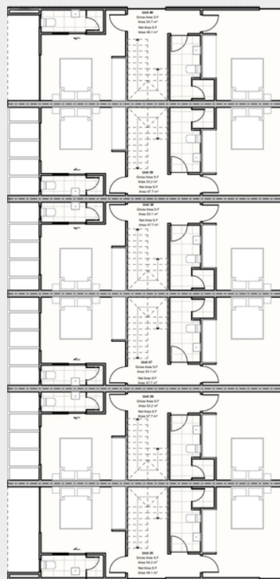
SECOND FLOOR UNITS 35 - 40
