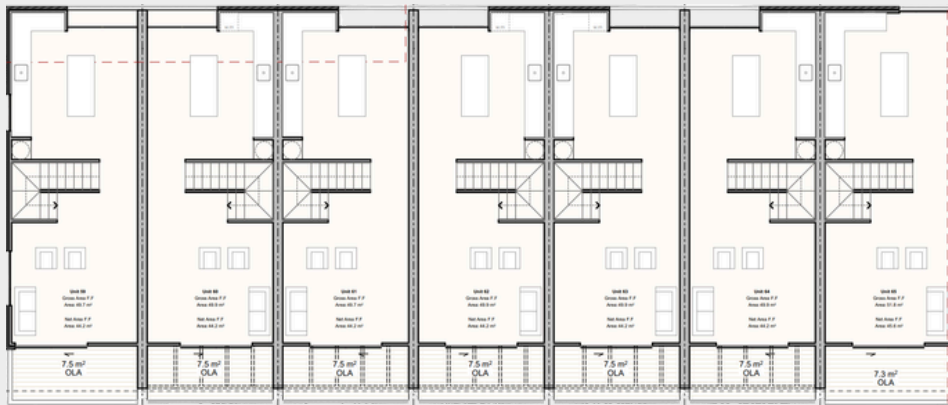
SECOND FLOOR UNITS 59 - 65
