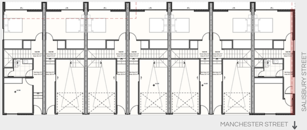
GROUND FLOOR UNITS 59 - 65
